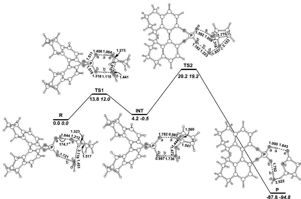
Figure 8. The optimized structures with selected bond lengths (in Å) of the reactant complex ( R ), the transition states (TS1 and TS2), the intermediate (INT) and the product ( P ). The geometries were fully optimized at the B3LYP/6-311+G** level. The relative free energies \Delta G_{\text{B3LYP-Sol}} (in bold) and \Delta G_{\text{MP2-Sol}} (in italic) are in kcal mol -1 .
