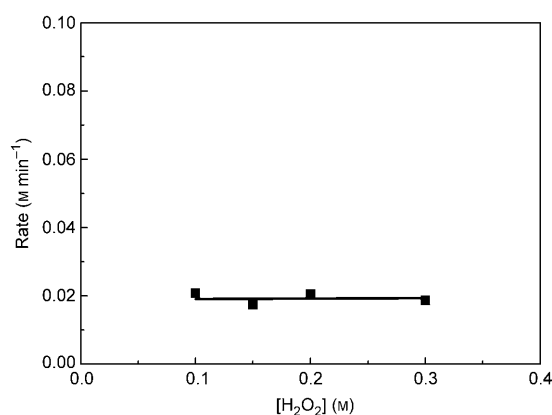
Figure 4. Plot of initial rate against [\text{H}_2\text{O}_2] in the presence of 1b (5 mM) at 27 °C (300 K) ( [2b] = 0.1 M in \text{CH}_2\text{Cl}_2 ).
