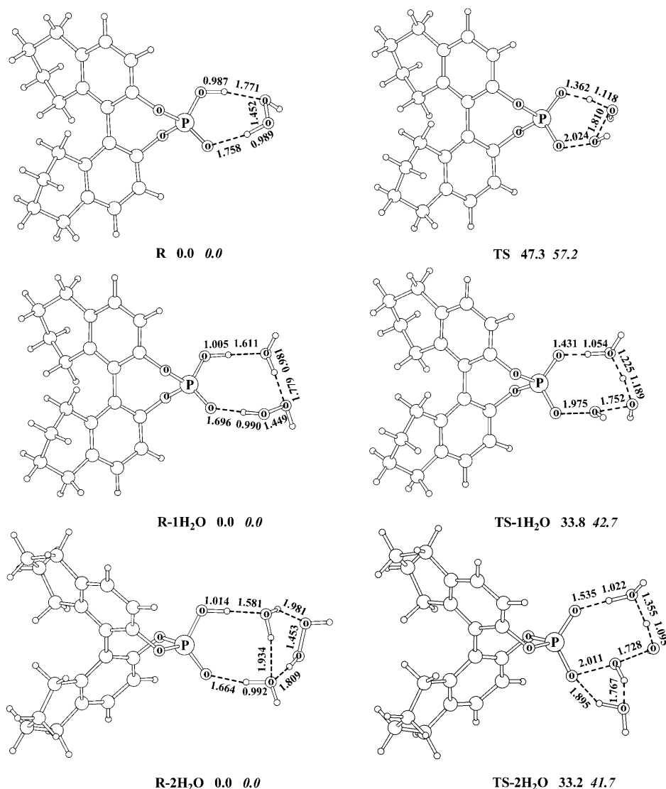
Figure 2. The optimized structures with selected bond lengths (in Å) of the reaction complex R and the corresponding transition states (TS) for the oxidation of the phosphoric acid 1c by hydrogen peroxide, with or without the assistance of water. The geometries were fully optimized at the B3LYP/6-311+G** level. The relative energies \Delta G_{\text{B3LYP-Sol}} (in bold) and \Delta G_{\text{MP2-Sol}} (in italic) are in kcal mol −1 (for the details of the calculation, see the Theoretical Calculations section).
