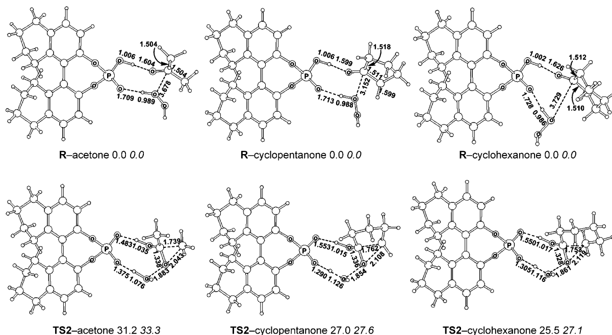
Figure 9. The calculated structures with selected bond lengths (in Å) and relative energies (in kcal mol −1 ) ( \Delta G_{B3LYP-Sol} (in bold) and \Delta G_{MP2-Sol} (in italic)) of the reactant complexes ( R ) and the transition states TS2 for the B–V reactions of acetone, cyclopentanone and cyclohexanone.
