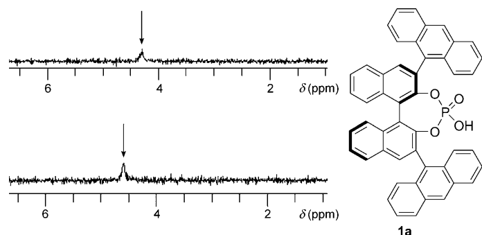
Figure 1. Comparison of ^{31}P NMR spectra of the phosphoric acid 1a in the presence (top; \delta = 4.292 ppm) or absence of H_2O_2 (bottom; \delta = 4.579 ppm).
