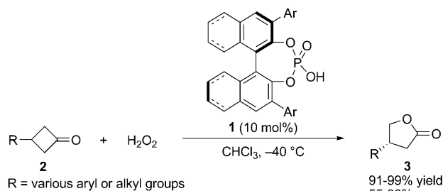
Scheme 1. BINOL-derived chiral phosphoric acid catalyzed enantioselective B–V reaction of cyclobutanone derivatives.
