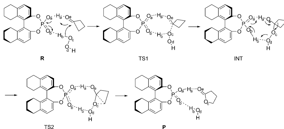
Scheme 5. Proposed two-step mechanism for the phosphoric acid ( \mathbf{1c} ) catalyzed B–V reaction.
