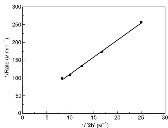
Figure 7. The Lineweaver–Burk plot of the B–V reaction of 2b in the presence of \text{H}_2\text{O}_2 (0.15 M) and 1b (2.5 mM) in \text{CH}_2\text{Cl}_2 at 300 K. y = 9.59x + 14.92 ; R^2 = 0.9973 .
