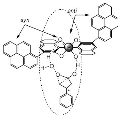
Scheme 6. The model used to calculate the enantioselectivity (6-311+G** basis set for the part of the structure encircled in the dashed line, but not including the binaphthyl backbone atoms, and the 6-31G* basis set for the remaining part).
