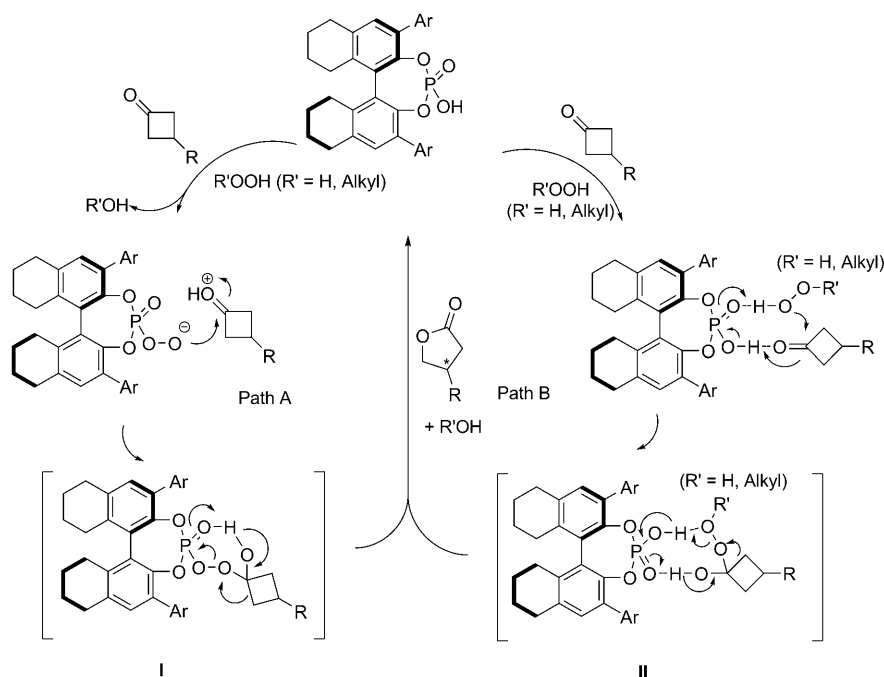
Scheme 2. Two plausible pathways for the chiral phosphoric acid catalyzed B–V oxidation of 3-substituted cyclobutanones by using R'OOH ( R' = H or alkyl) as oxidants.
