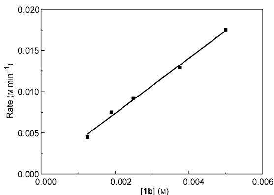
Figure 5. Plot of initial rate of 2b (0.1 M in \text{CH}_2\text{Cl}_2 ) with \text{H}_2\text{O}_2 (0.15 M) against [1b] (1.25 to 5 mM) at 27 °C (300 K). y = 3.34428x + 0.00069 , R^2 = 0.9936 .
