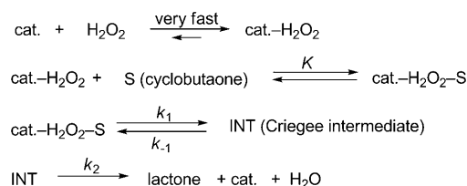
Scheme 4. A refined catalytic cycle based on kinetic studies.
